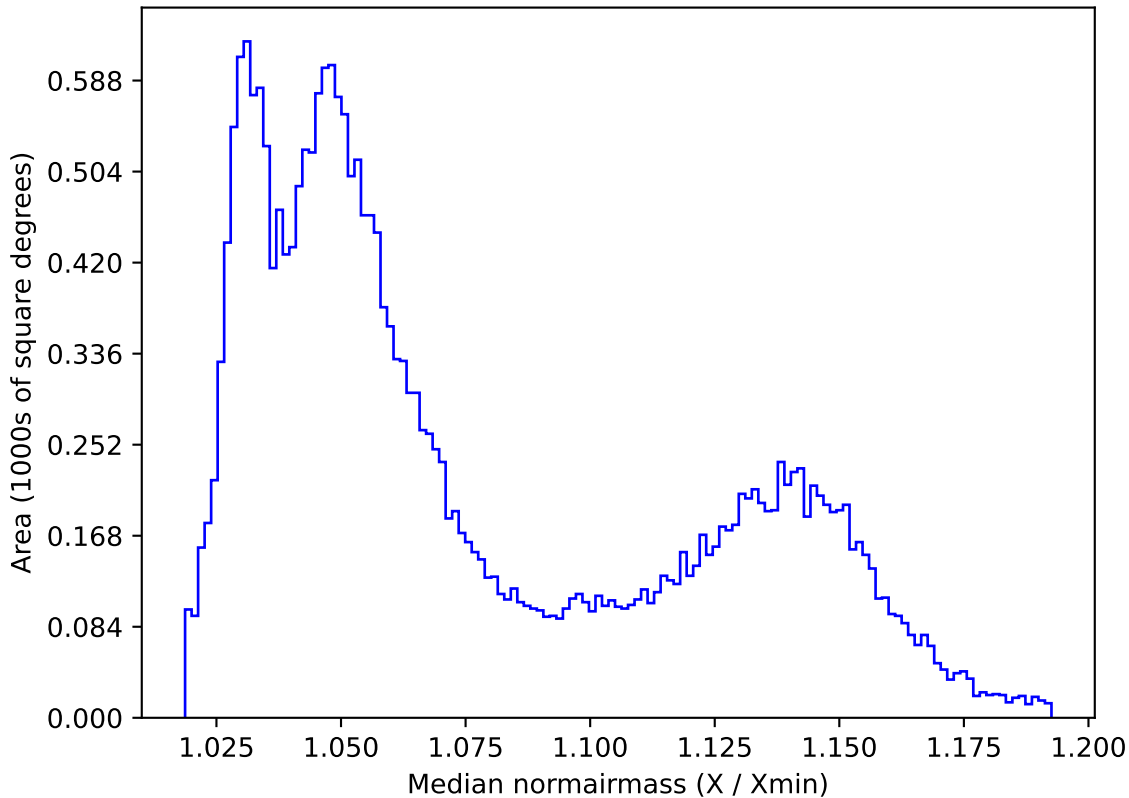
early_u_fpextra2.0_v3.4_10yrs All sky all bands: Median normairmass
