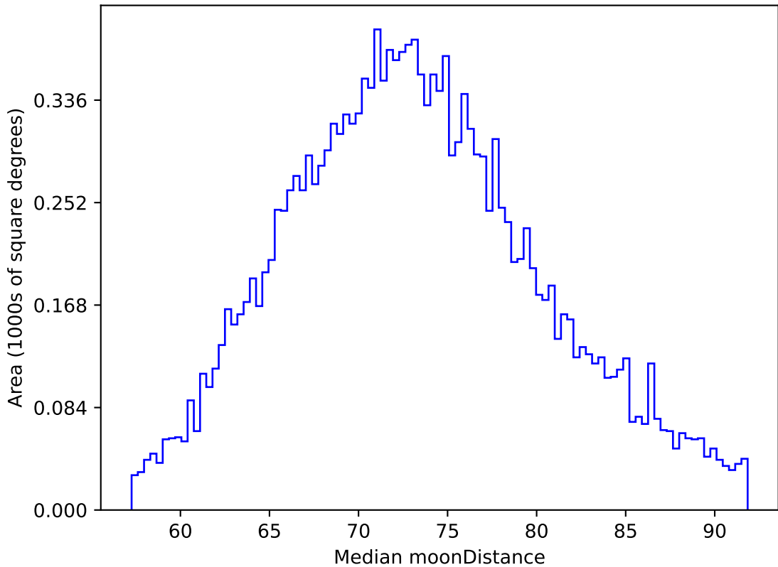
early_u_fpextra2.0_v3.4_10yrs WFD z band: Median moonDistance
