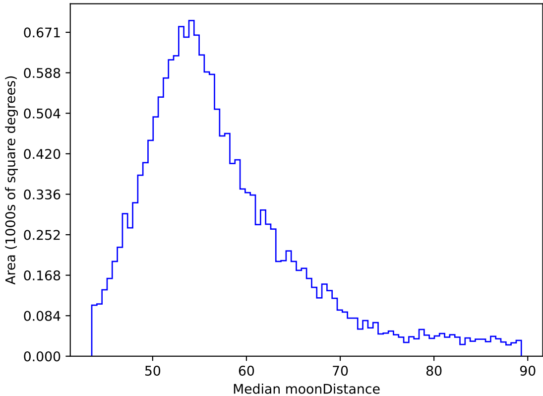
early_u_fpextra2.0_v3.4_10yrs WFD y band: Median moonDistance
