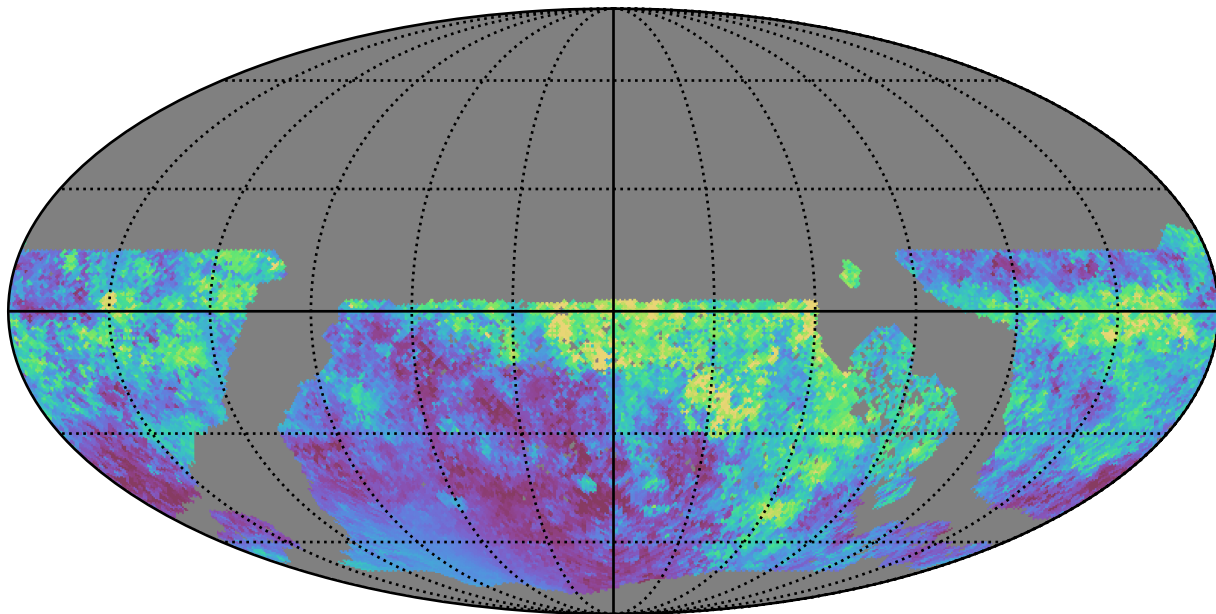
early_u_fpextra2.0_v3.4_10yrs WFD i band: Median moonDistance
