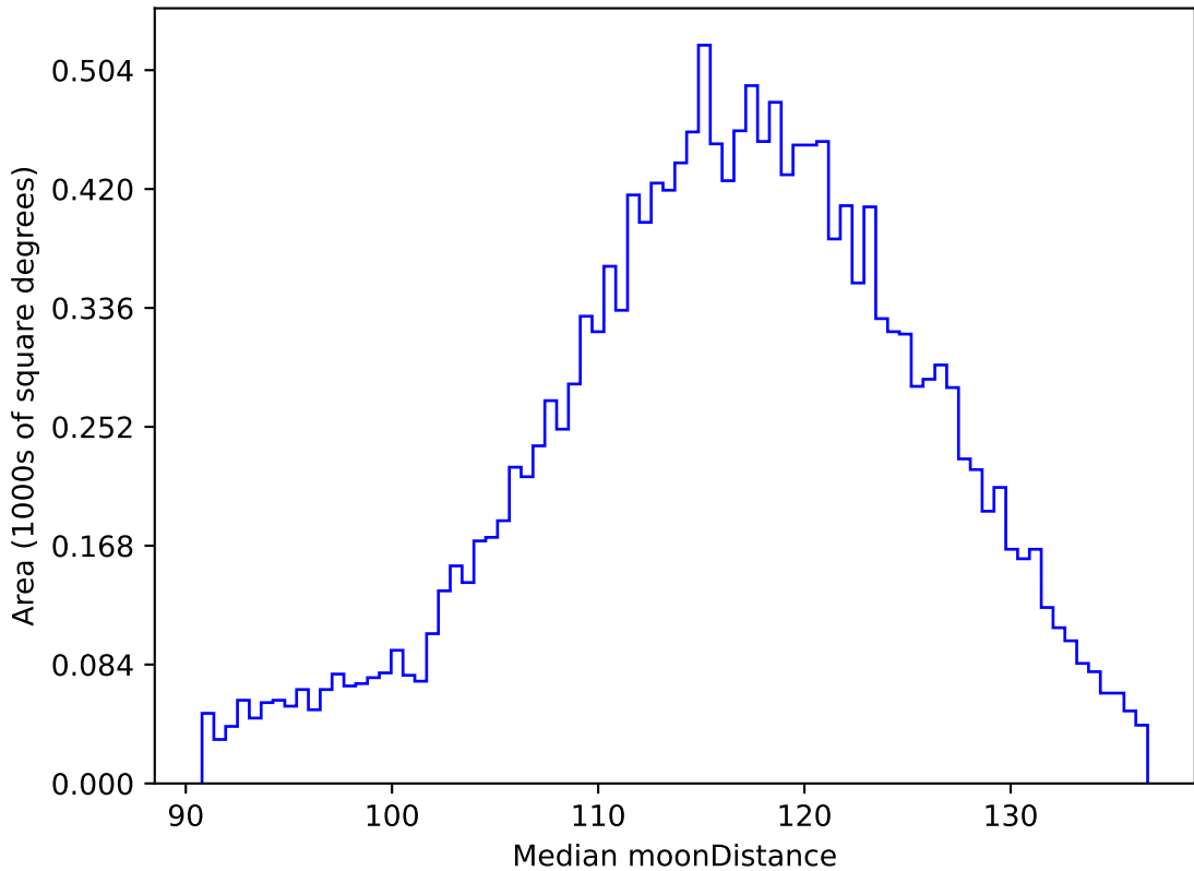
early_u_fpextra2.0_v3.4_10yrs WFD g band: Median moonDistance
