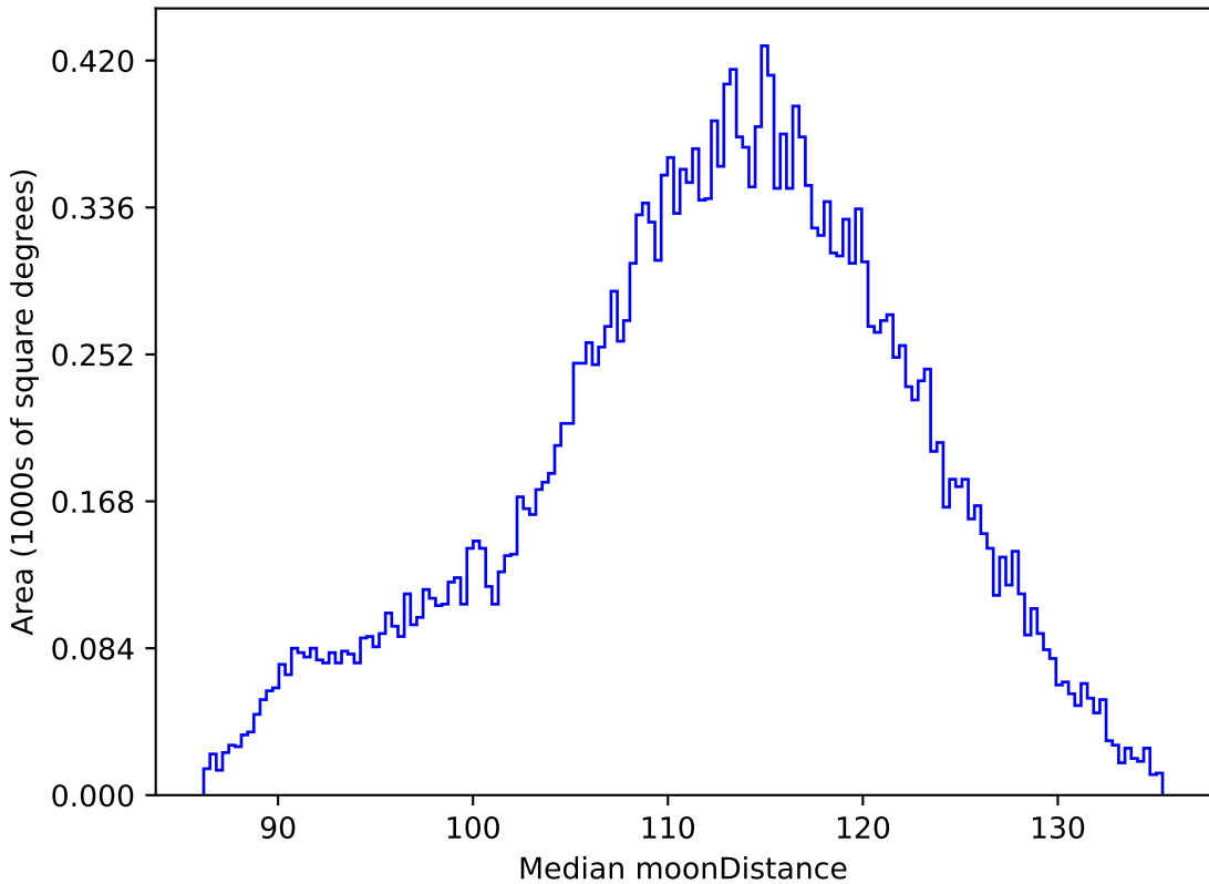
early_u_fpextra2.0_v3.4_10yrs All sky r band: Median moonDistance
