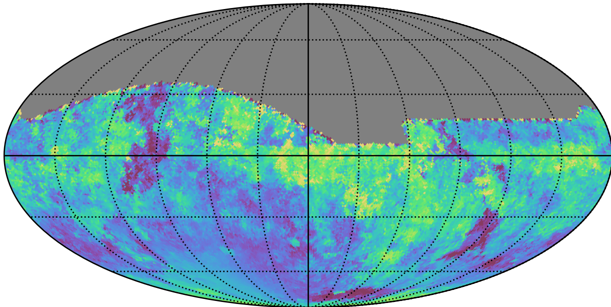
early_u_fpextra2.0_v3.4_10yrs All sky i band: Median moonDistance
