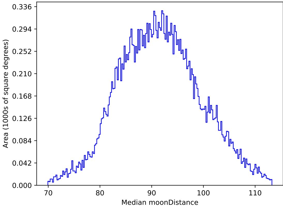
early_u_fpextra2.0_v3.4_10yrs All sky i band: Median moonDistance
