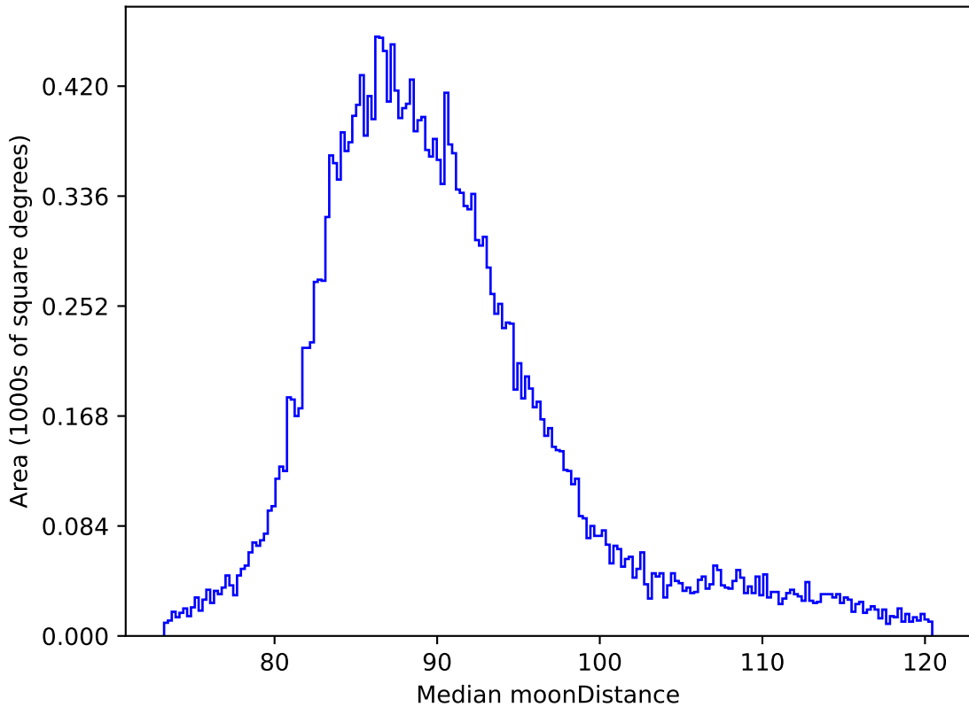
early_u_fpextra2.0_v3.4_10yrs All sky all bands: Median moonDistance
