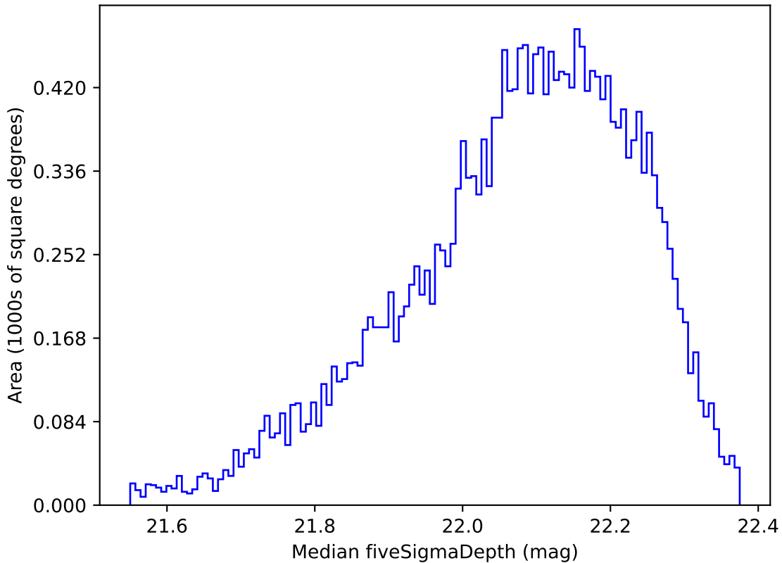
early_u_fpextra2.0_v3.4_10yrs Yr 1 y band: Median fiveSigmaDepth
