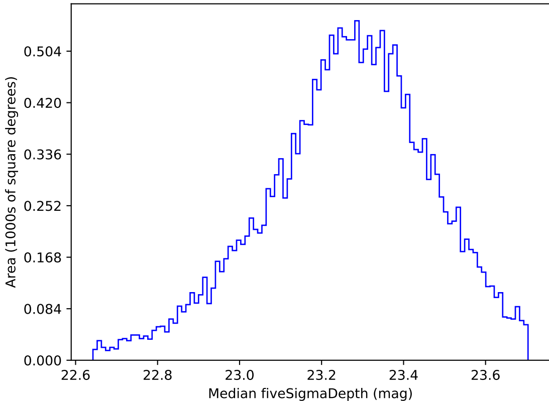
early_u_fpextra2.0_v3.4_10yrs Yr 1 u band: Median fiveSigmaDepth
