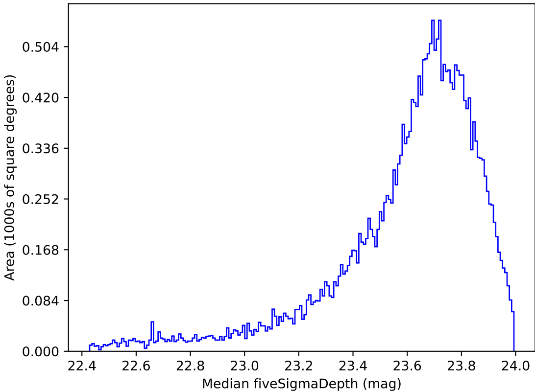
early_u_fpextra2.0_v3.4_10yrs Yr 1 i band: Median fiveSigmaDepth
