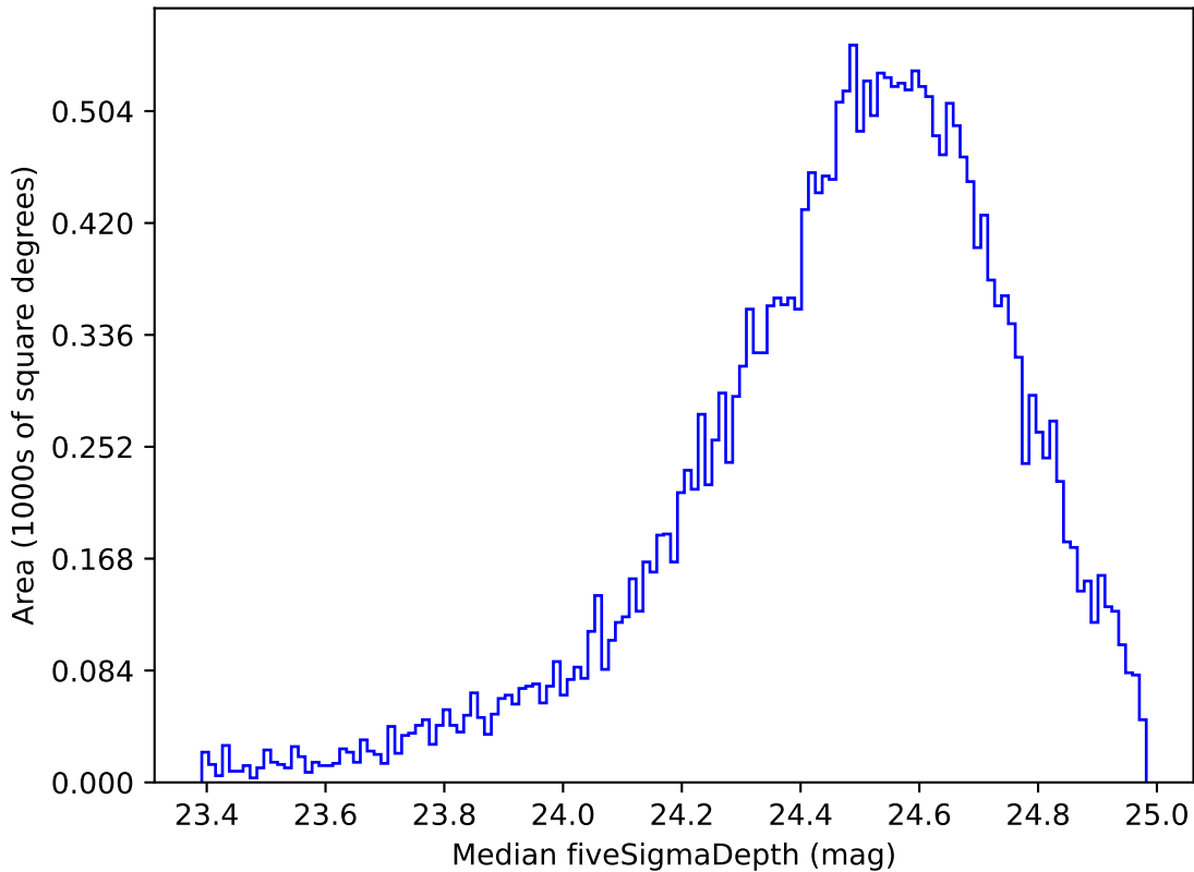
early_u_fpextra2.0_v3.4_10yrs Yr 1 g band: Median fiveSigmaDepth
