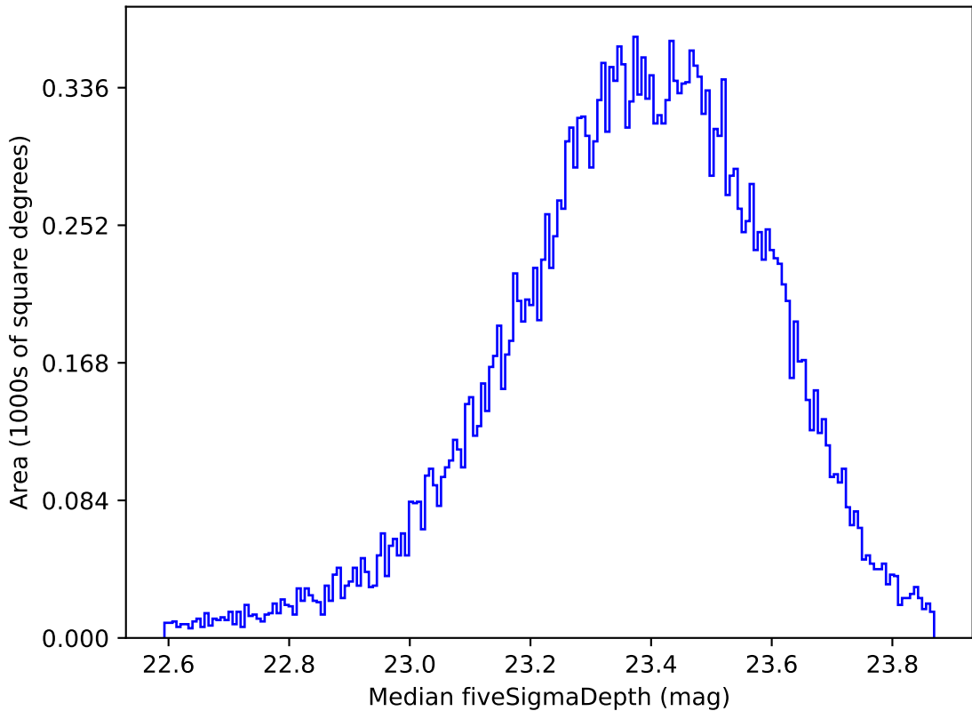
early_u_fpextra2.0_v3.4_10yrs Yr 1 all bands: Median fiveSigmaDepth
