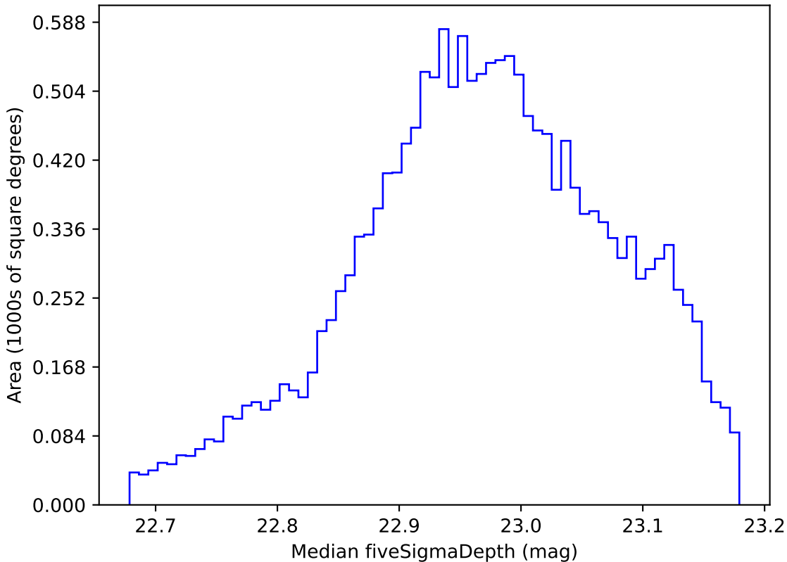
early_u_fpextra2.0_v3.4_10yrs WFD z band: Median fiveSigmaDepth
