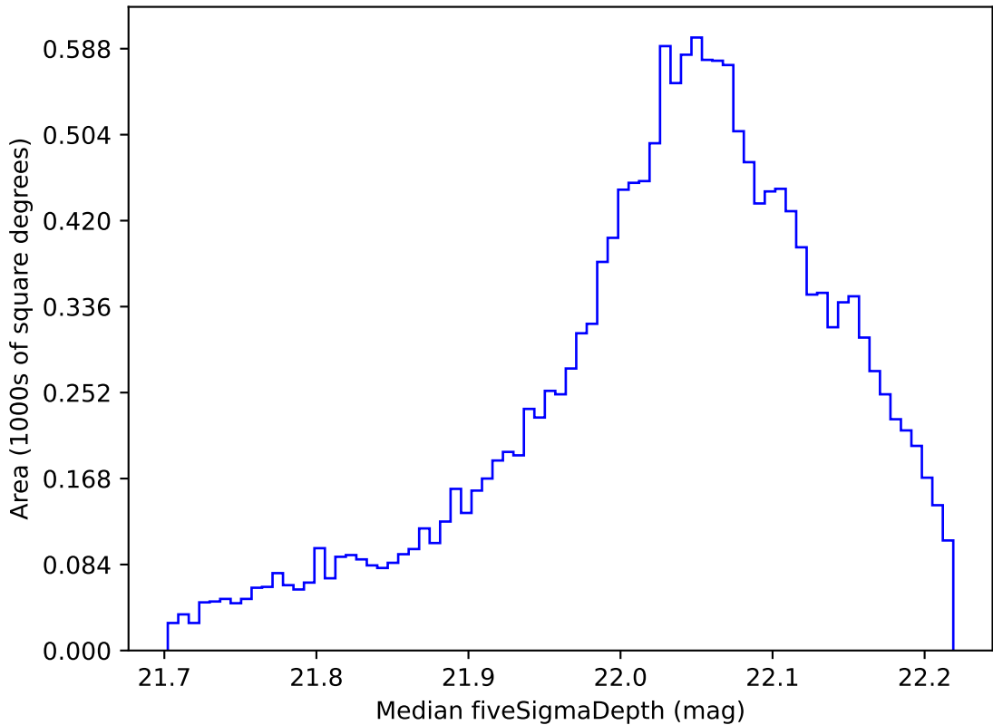
early_u_fpextra2.0_v3.4_10yrs WFD y band: Median fiveSigmaDepth
