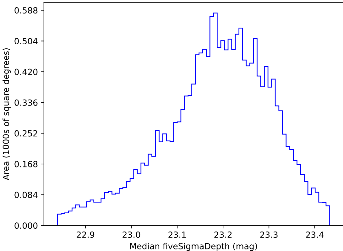
early_u_fpextra2.0_v3.4_10yrs WFD u band: Median fiveSigmaDepth
