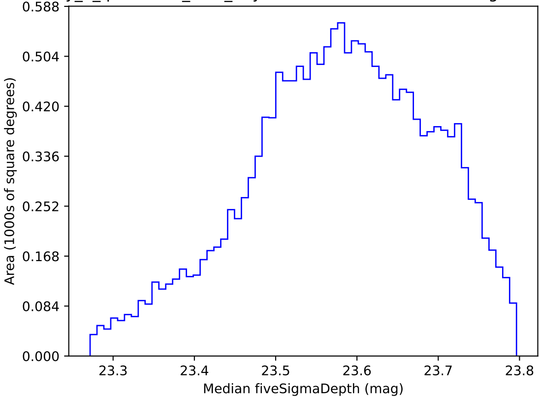
early_u_fpextra2.0_v3.4_10yrs WFD i band: Median fiveSigmaDepth
