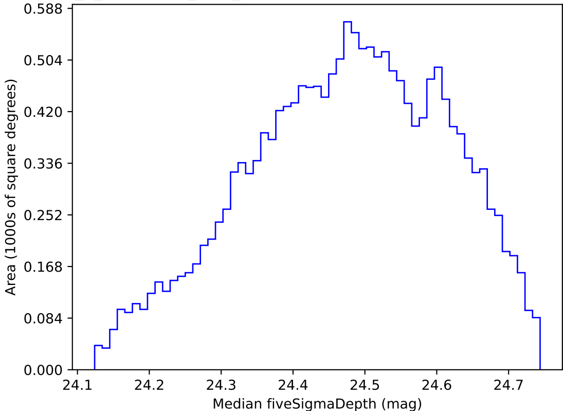
early_u_fpextra2.0_v3.4_10yrs WFD g band: Median fiveSigmaDepth
