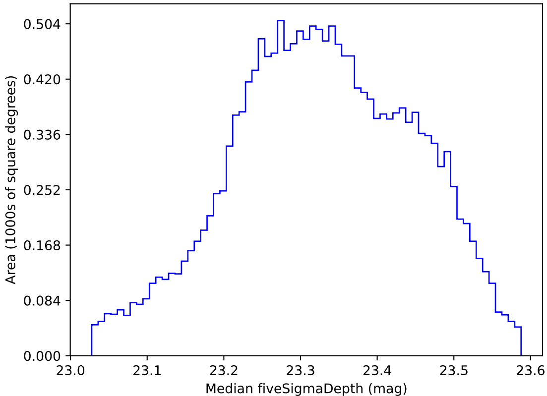
early_u_fpextra2.0_v3.4_10yrs WFD all bands: Median fiveSigmaDepth
