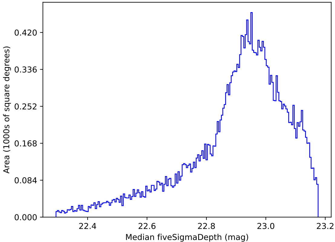
early_u_fpextra2.0_v3.4_10yrs All sky z band: Median fiveSigmaDepth
