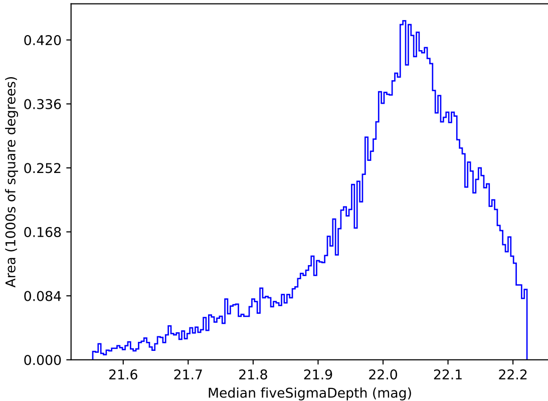
early_u_fpextra2.0_v3.4_10yrs All sky y band: Median fiveSigmaDepth
