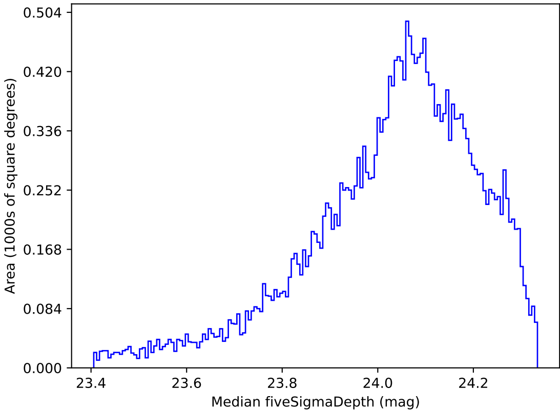
early_u_fpextra2.0_v3.4_10yrs All sky r band: Median fiveSigmaDepth
