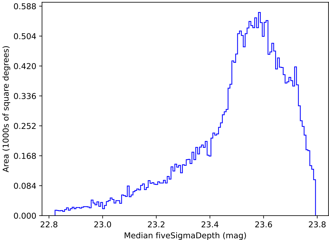
early_u_fpextra2.0_v3.4_10yrs All sky i band: Median fiveSigmaDepth
