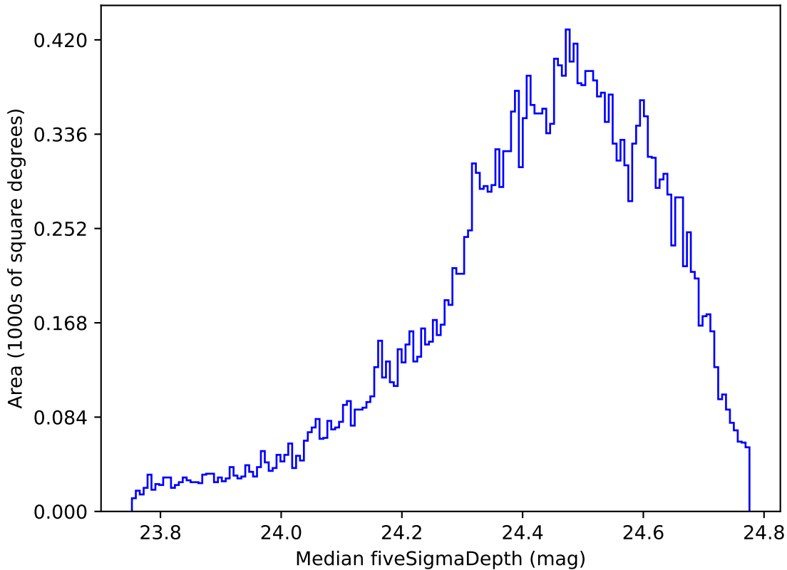
early_u_fpextra2.0_v3.4_10yrs All sky g band: Median fiveSigmaDepth
