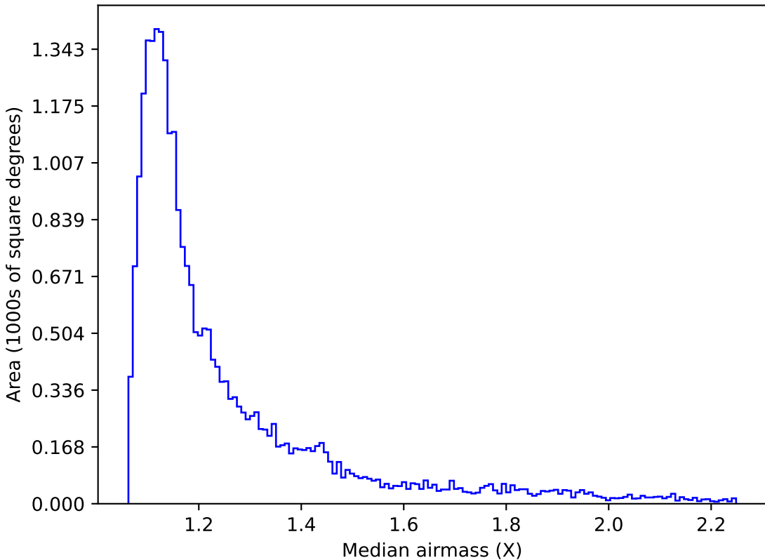
early_u_fpextra2.0_v3.4_10yrs Yr 1 z band: Median airmass
