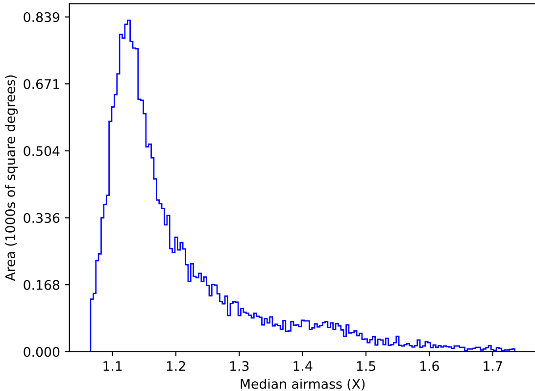
early_u_fpextra2.0_v3.4_10yrs Yr 1 y band: Median airmass
