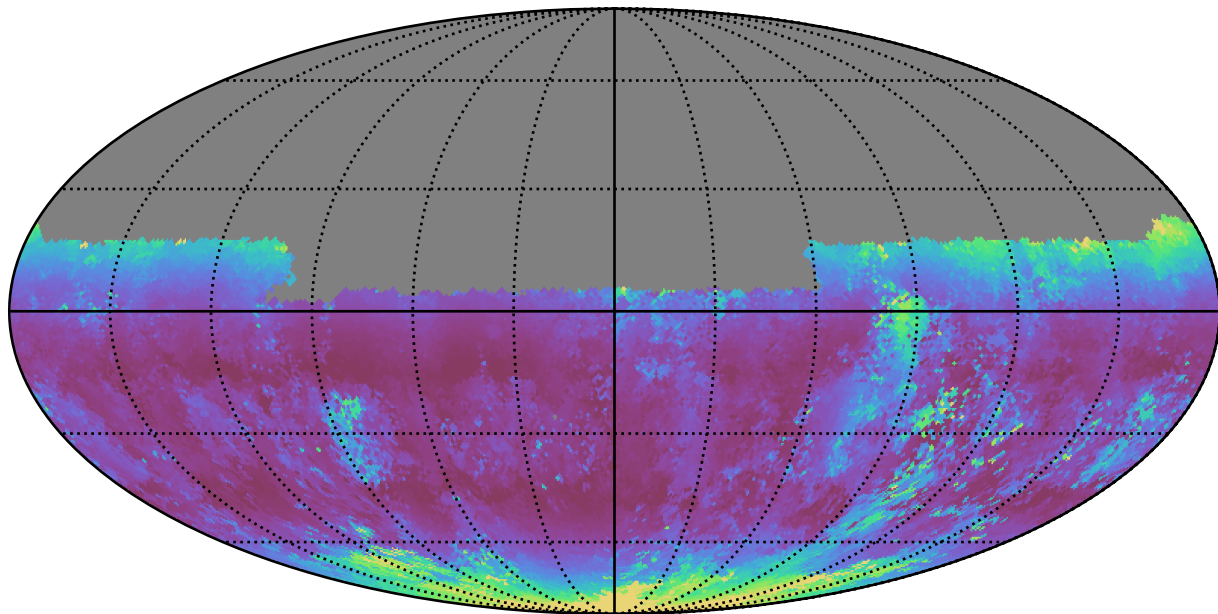
early_u_fpextra2.0_v3.4_10yrs Yr 1 u band: Median airmass
