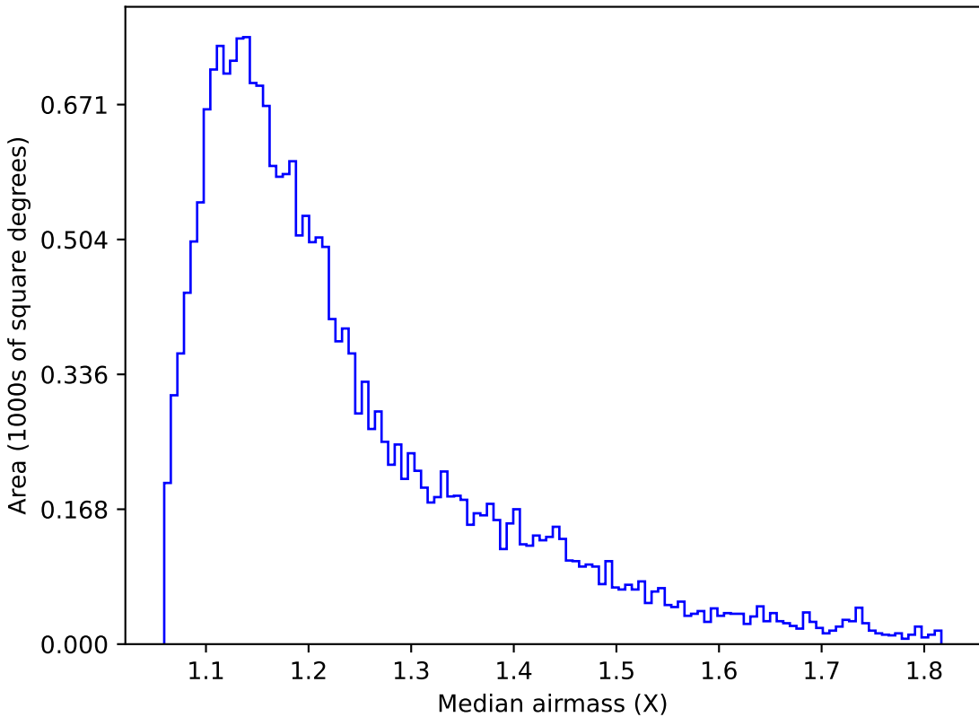
early_u_fpextra2.0_v3.4_10yrs Yr 1 u band: Median airmass
