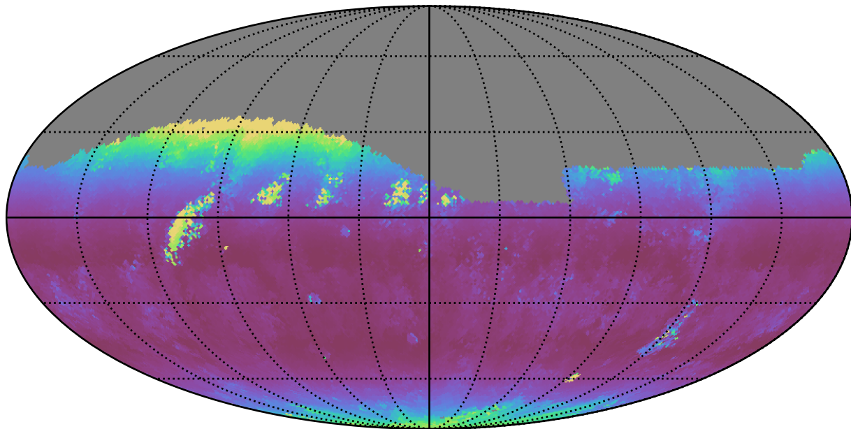
early_u_fpextra2.0_v3.4_10yrs Yr 1 r band: Median airmass
