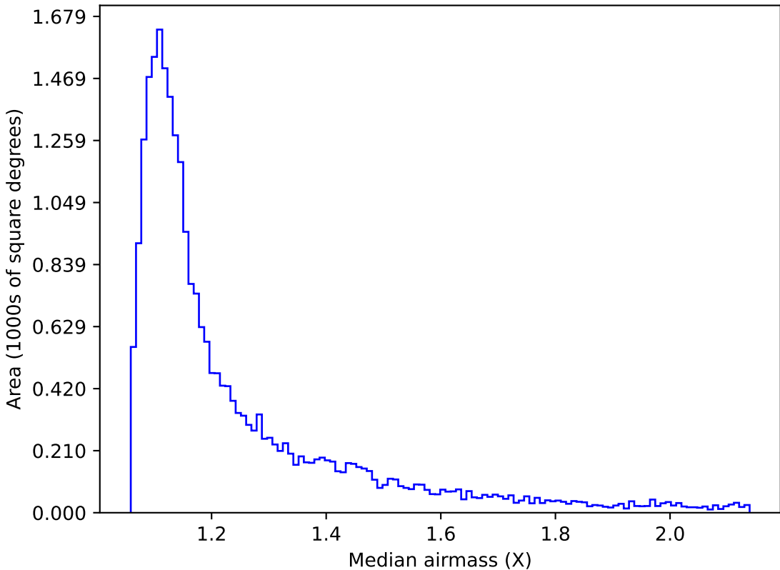
early_u_fpextra2.0_v3.4_10yrs Yr 1 r band: Median airmass
