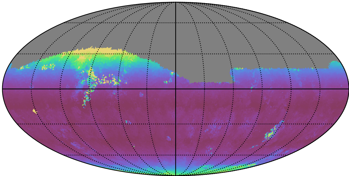
early_u_fpextra2.0_v3.4_10yrs Yr 1 i band: Median airmass
