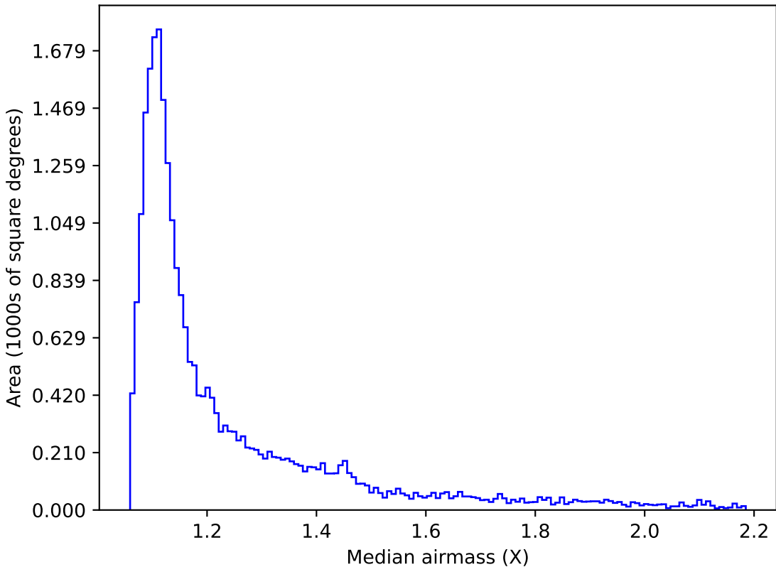
early_u_fpextra2.0_v3.4_10yrs Yr 1 i band: Median airmass
