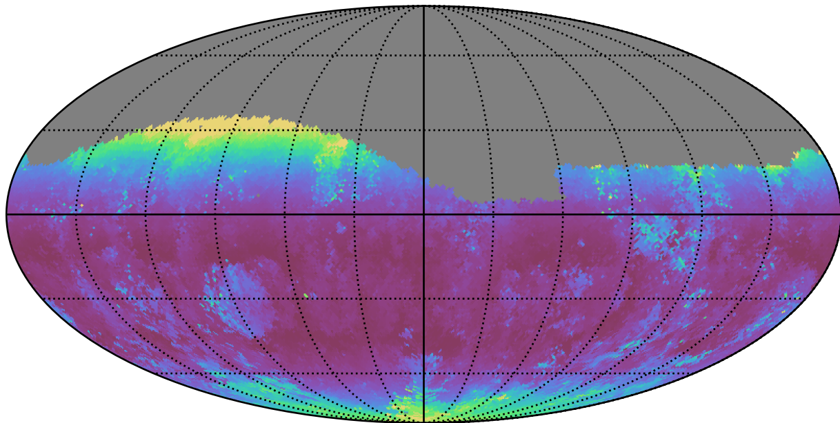
early_u_fpextra2.0_v3.4_10yrs Yr 1 g band: Median airmass
