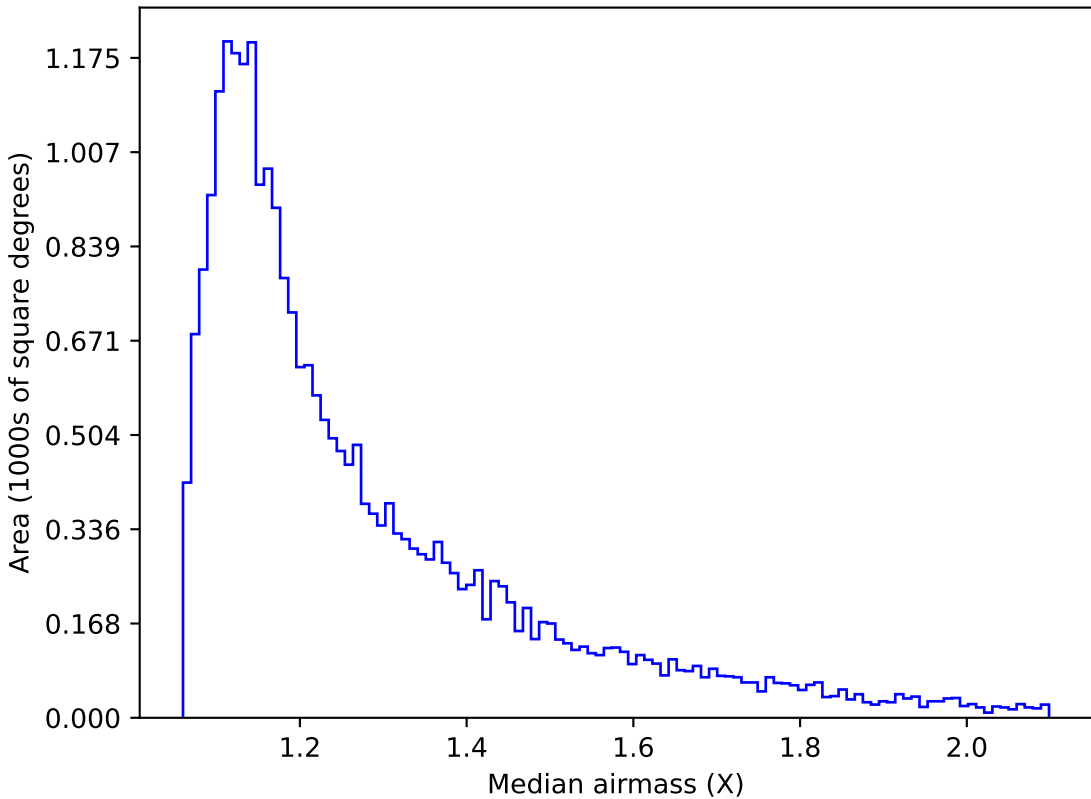
early_u_fpextra2.0_v3.4_10yrs Yr 1 g band: Median airmass
