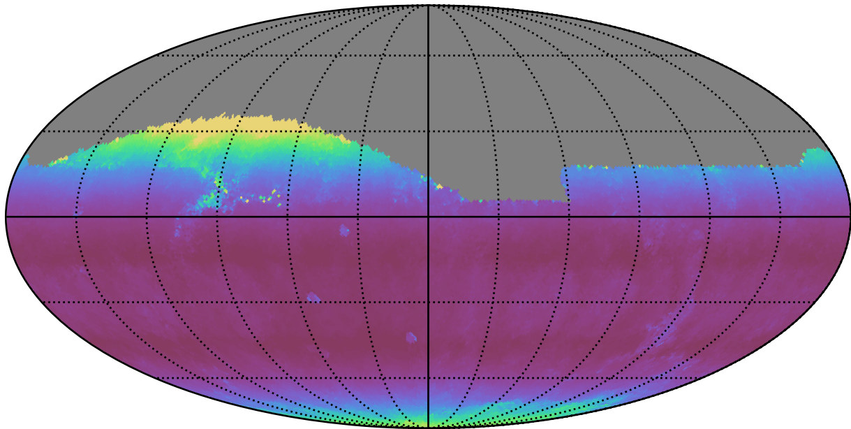
early_u_fpextra2.0_v3.4_10yrs Yr 1 all bands: Median airmass
