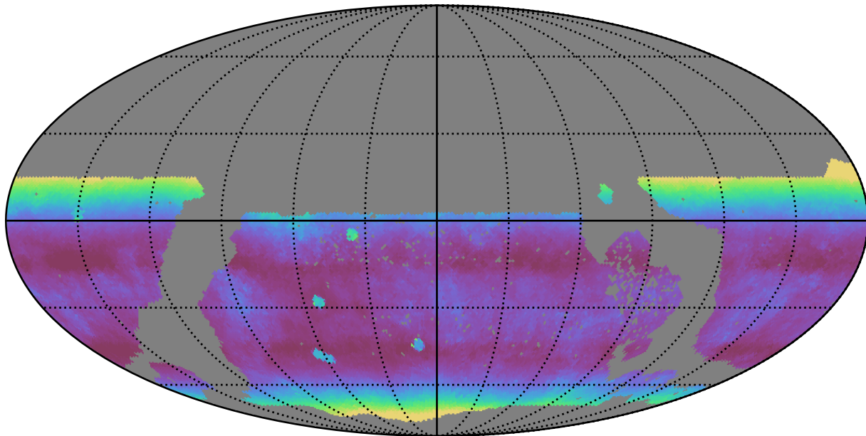
early_u_fpextra2.0_v3.4_10yrs WFD z band: Median airmass
