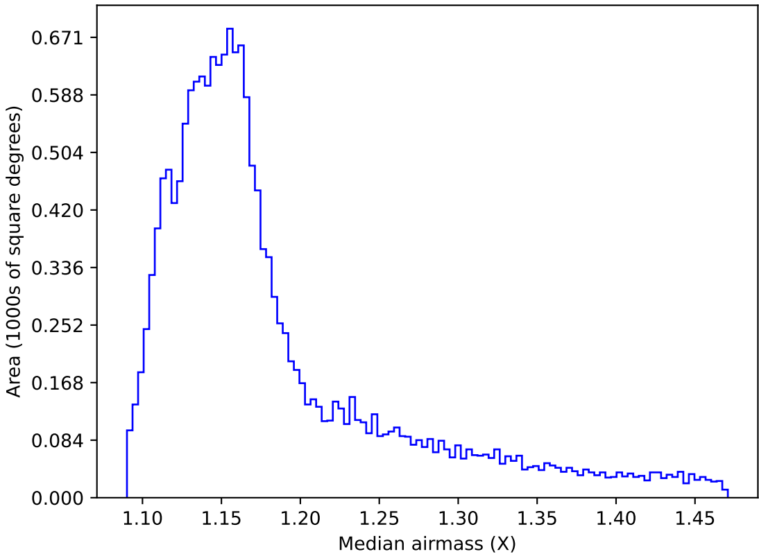
early_u_fpextra2.0_v3.4_10yrs WFD z band: Median airmass
