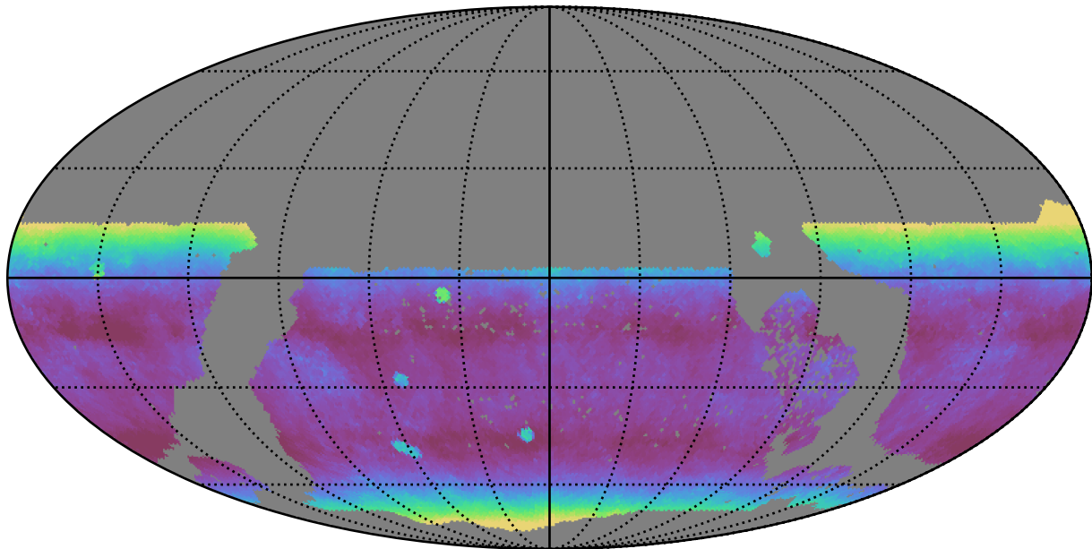
early_u_fpextra2.0_v3.4_10yrs WFD y band: Median airmass
