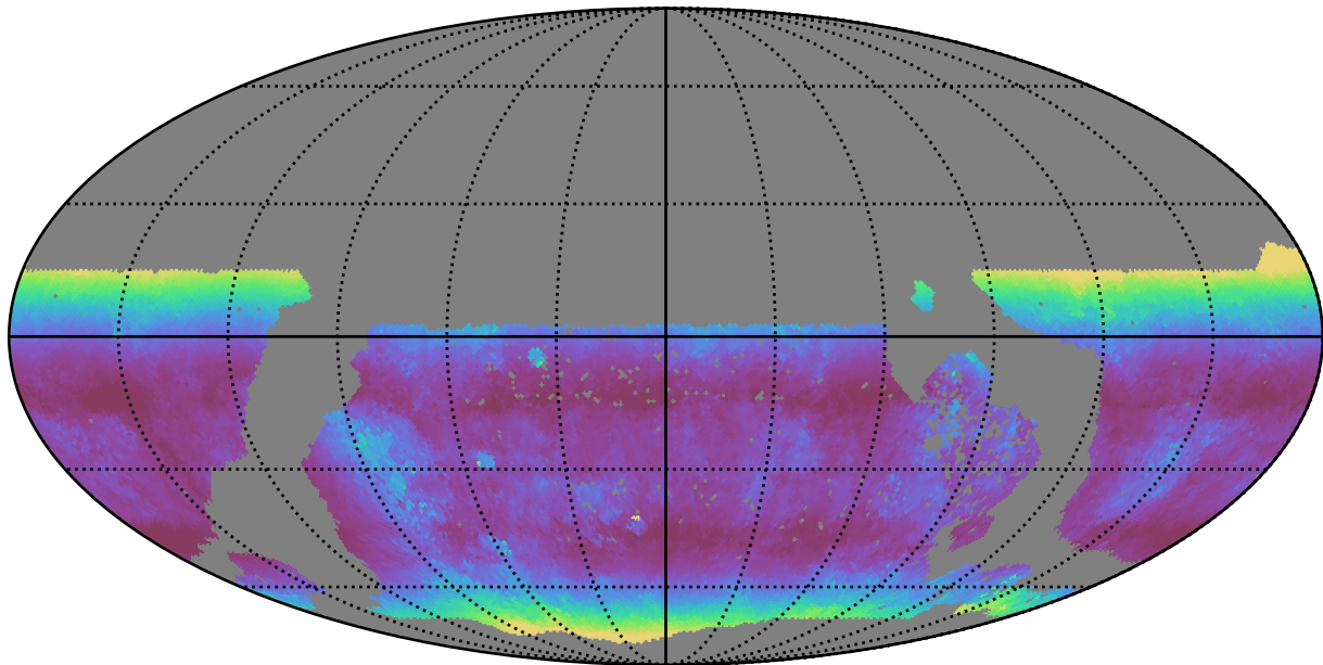
early_u_fpextra2.0_v3.4_10yrs WFD u band: Median airmass
