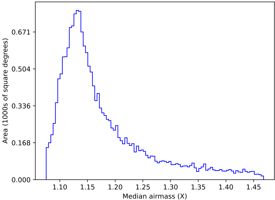
early_u_fpextra2.0_v3.4_10yrs WFD u band: Median airmass
