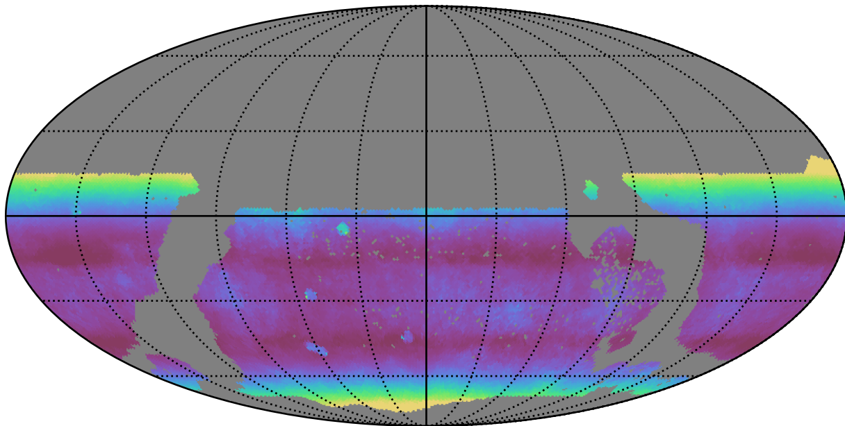
early_u_fpextra2.0_v3.4_10yrs WFD i band: Median airmass
