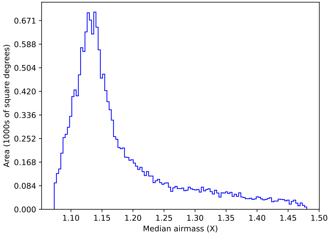
early_u_fpextra2.0_v3.4_10yrs WFD g band: Median airmass
