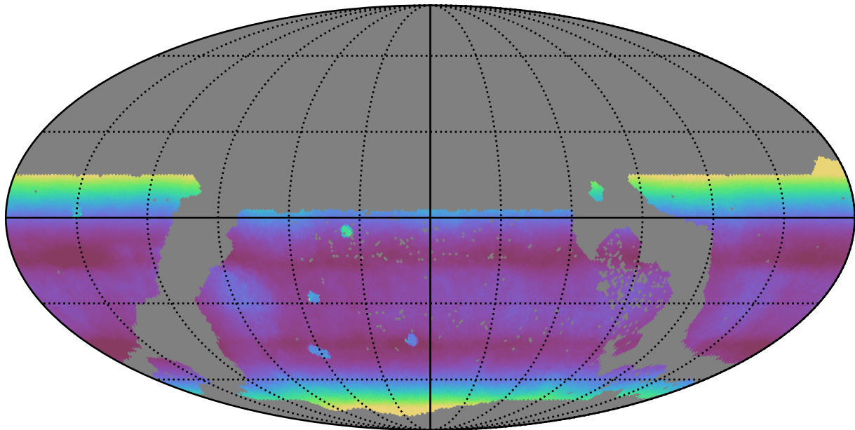
early_u_fpextra2.0_v3.4_10yrs WFD all bands: Median airmass
