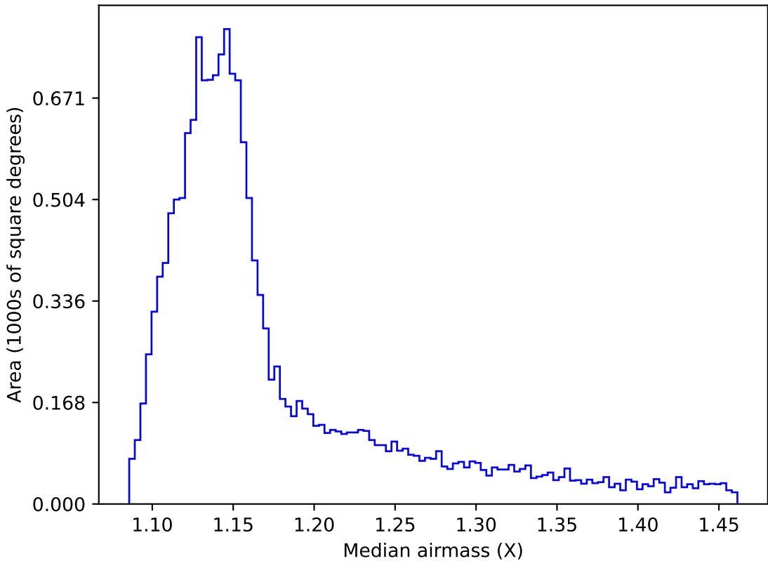
early_u_fpextra2.0_v3.4_10yrs WFD all bands: Median airmass
