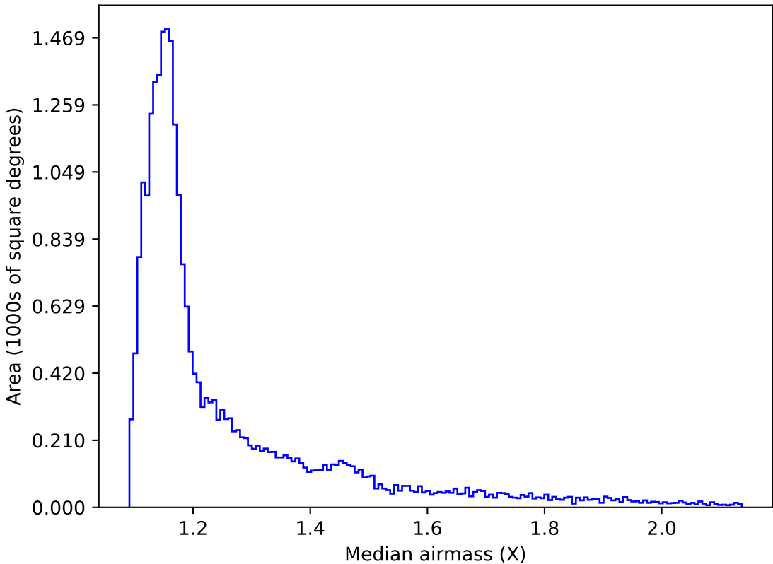
early_u_fpextra2.0_v3.4_10yrs All sky z band: Median airmass
