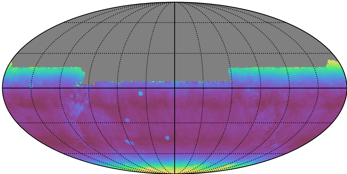
early_u_fpextra2.0_v3.4_10yrs All sky y band: Median airmass
