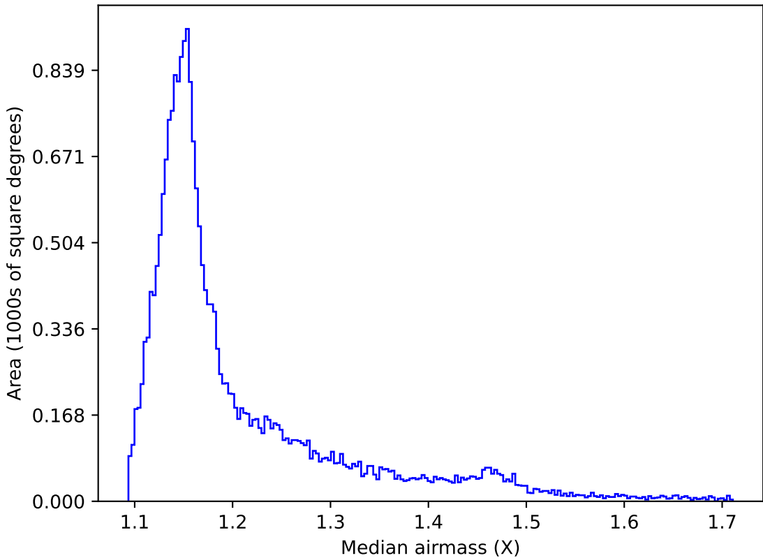
early_u_fpextra2.0_v3.4_10yrs All sky y band: Median airmass
