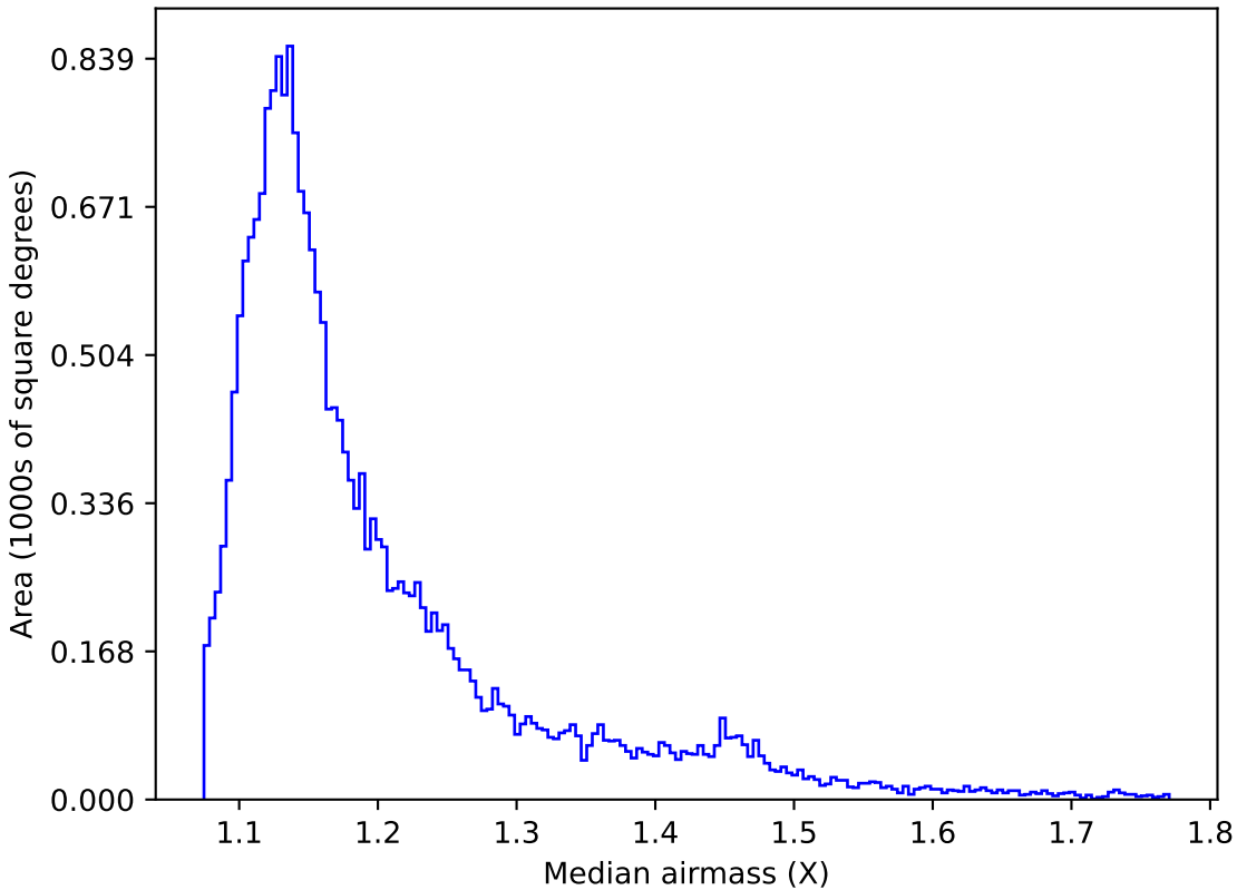
early_u_fpextra2.0_v3.4_10yrs All sky u band: Median airmass
