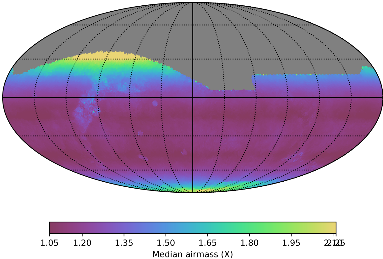
early_u_fpextra2.0_v3.4_10yrs All sky i band: Median airmass
